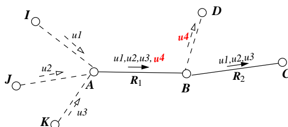
Figure 3.1. An Example of Inference-Route Problem
