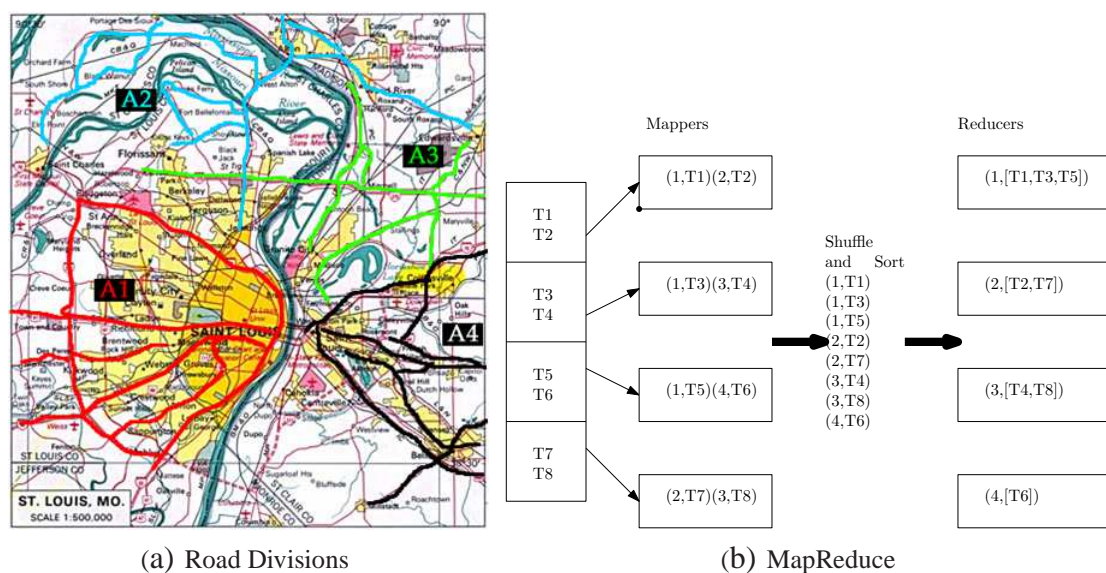
Figure 4.1. MapReduce Architecture
