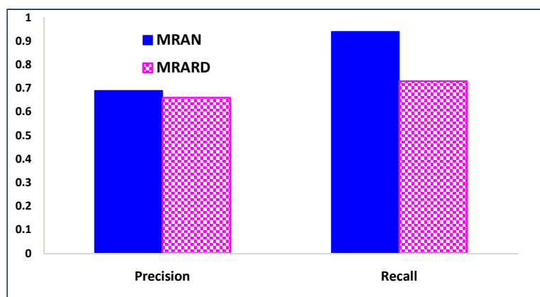
Figure 4.6. MapReduce-Based Approaches
