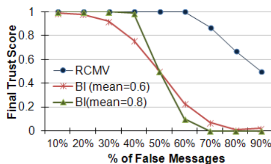
Figure 5.3. RCMV vs. BI
